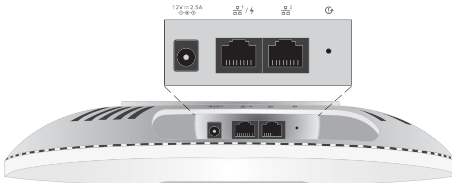
Figure 2. Hardware interfaces
