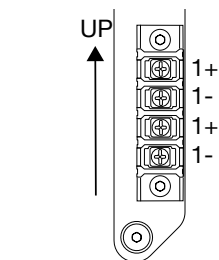
Screw terminal input/link wiring
