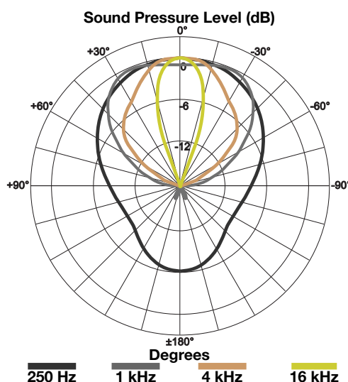
Vertical Polar Plot
