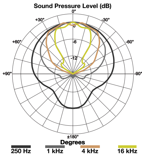
Horizontal Polar Plot
